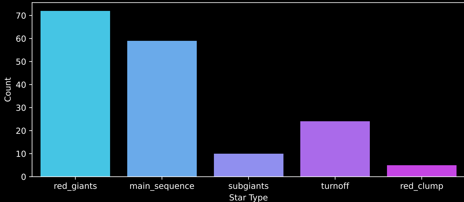
APOGEE DR17 Field: [274-21-O_TESS] Count plot of Star Type
