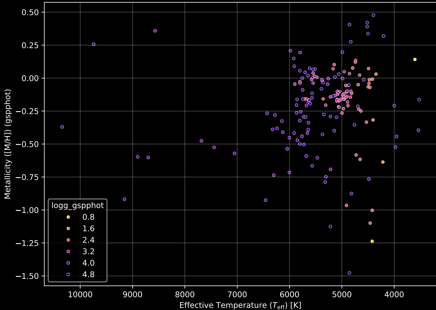
APOGEE DR17 Field: [274-21-O_TESS] Stellar Population Parameters (n= 170)
