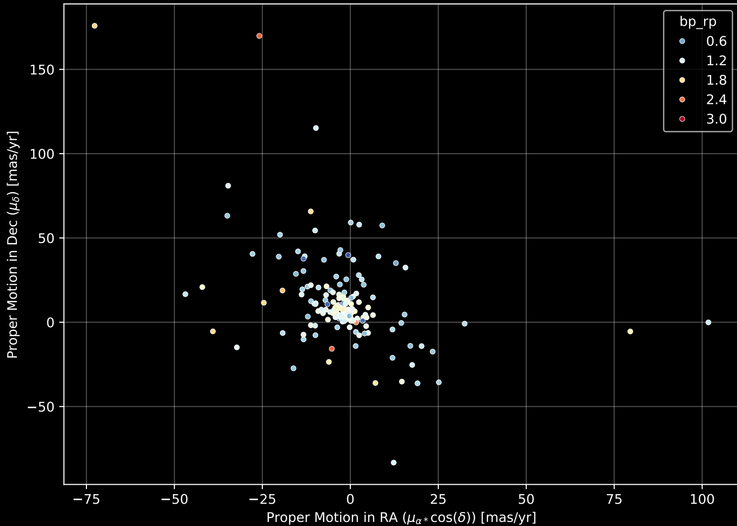
APOGEE DR17 Field: [274-21-O_TESS] Proper Motion Diagram (n= 170)
