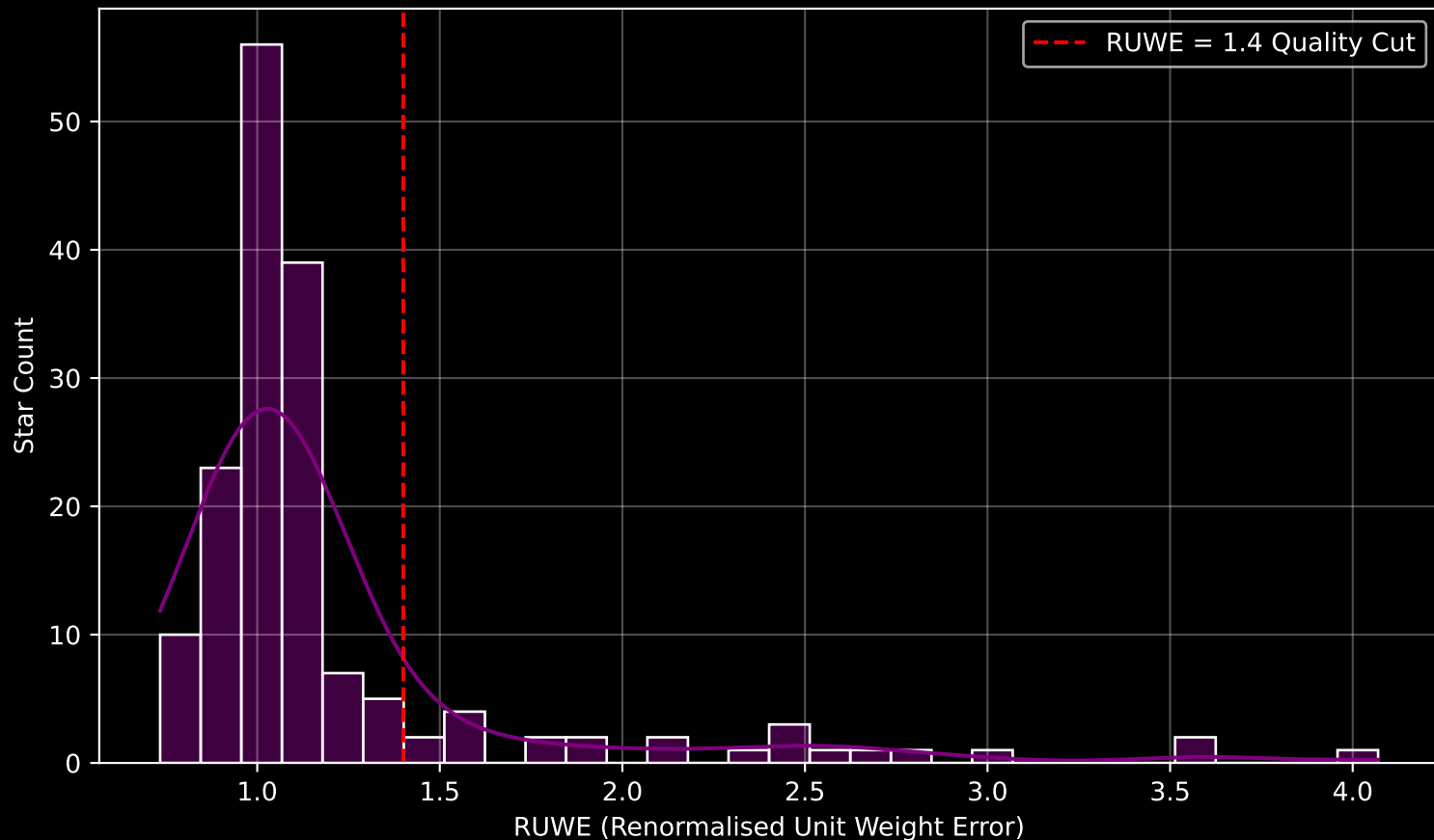
GAPOGEE DR17 Field [274-21-O_TESS] RUWE Distribution (n= 163)
