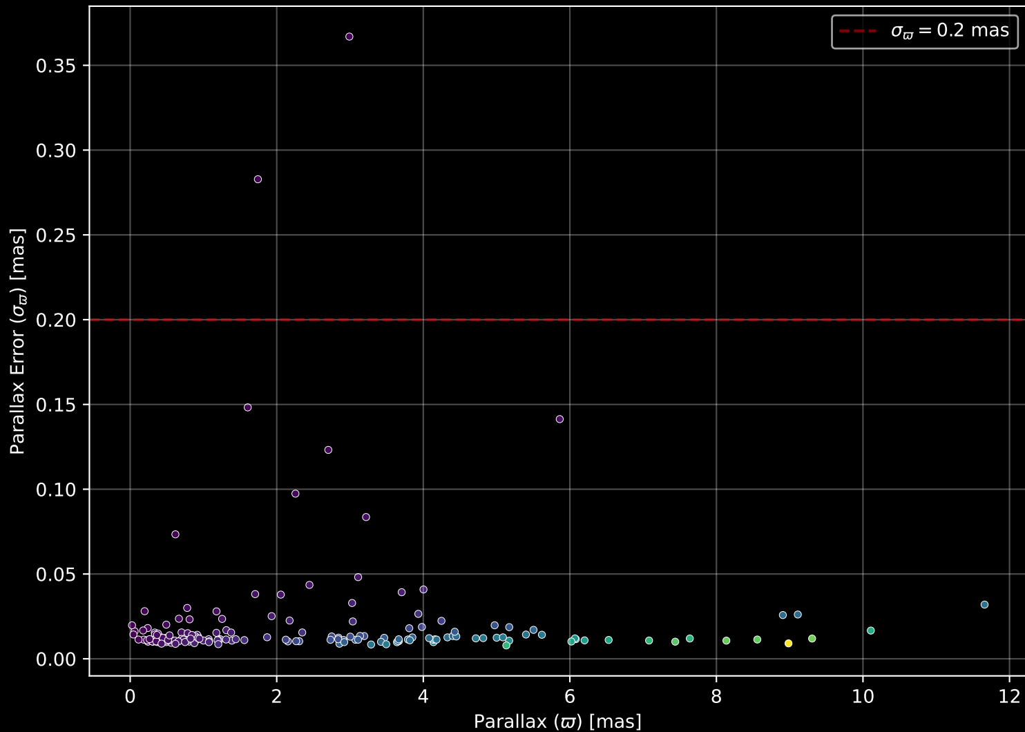
APOGEE DR17 Field: [274-21-O_TESS] Parallax Quality (n= 170)
