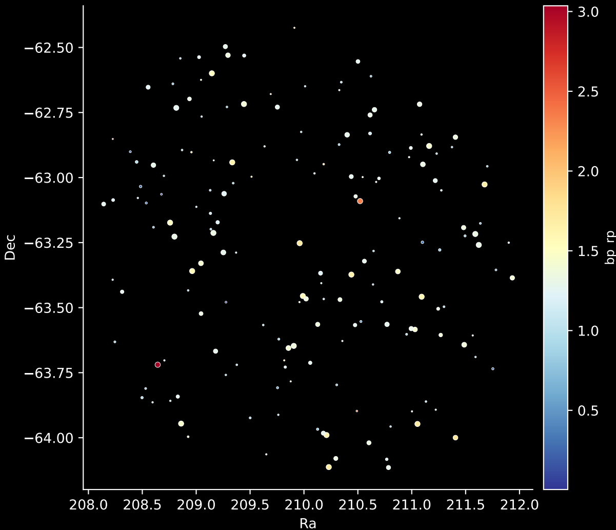
APOGEE DR17 Field: [274-21-O_TESS] Stars: 170
